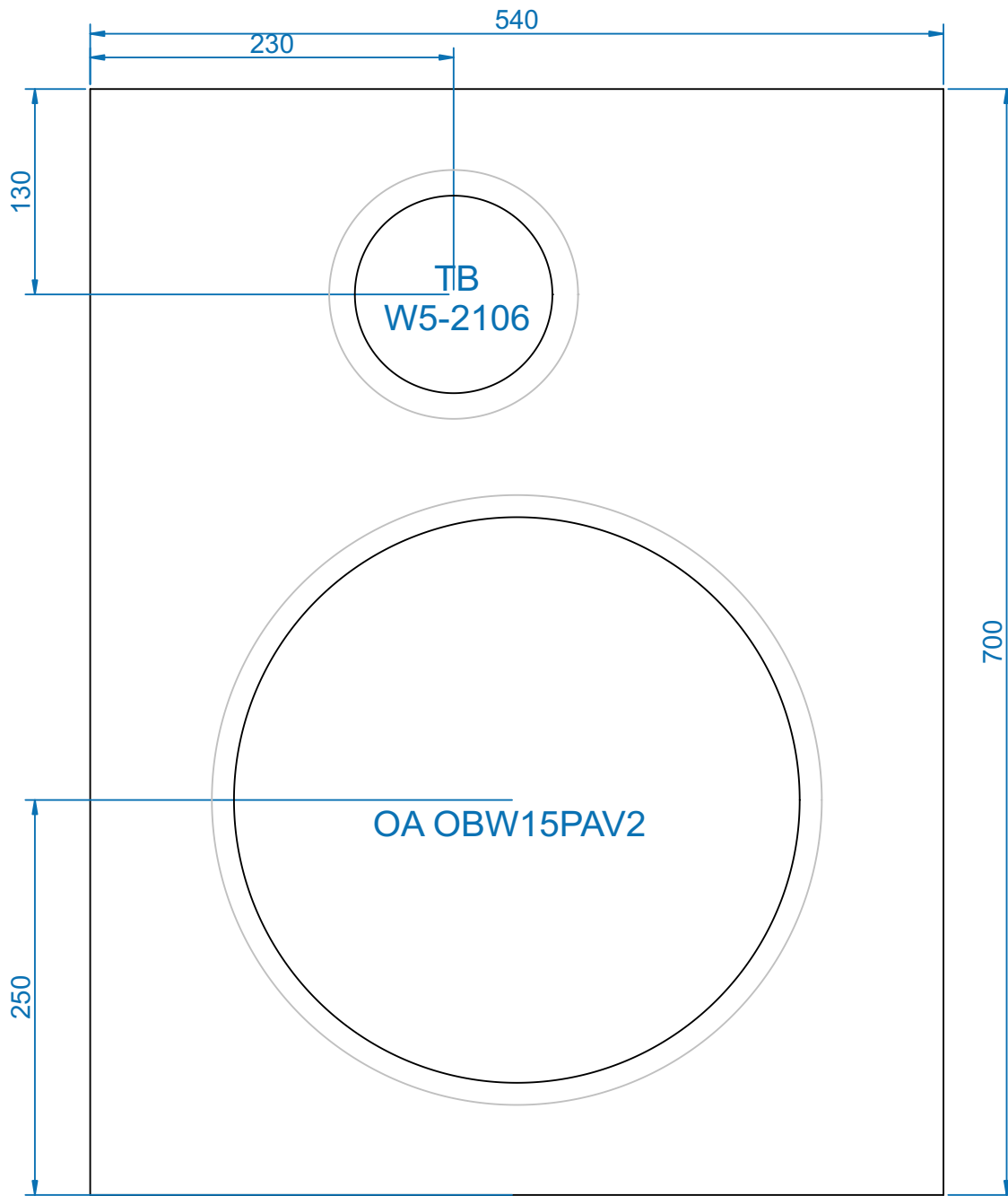
PowerDuo W5-2106 (c)Niklas Baur, blue planet acoustic
