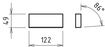
Port Panel
