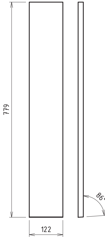
Divider Panel
