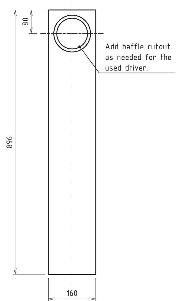
Front Panel
